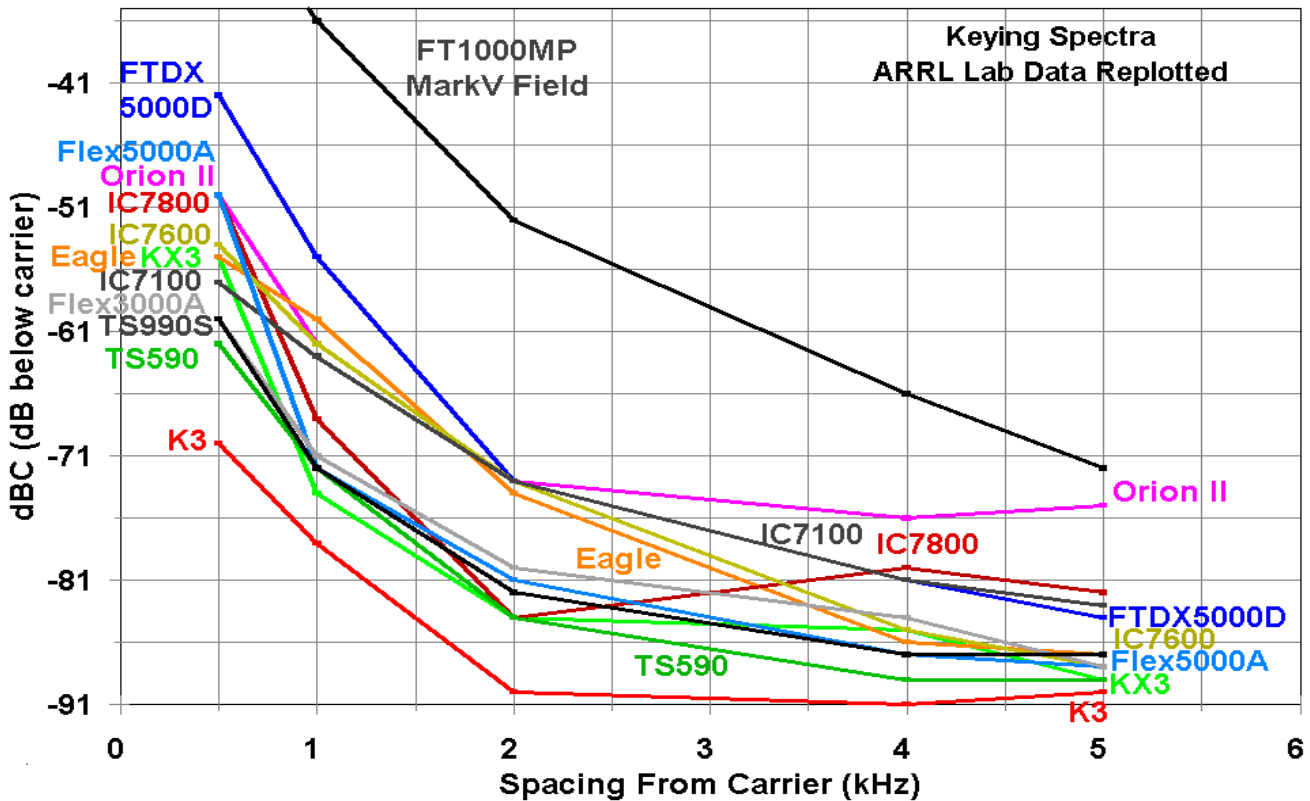
Figure 2 – The Rigs Compared For CW Spectrum
