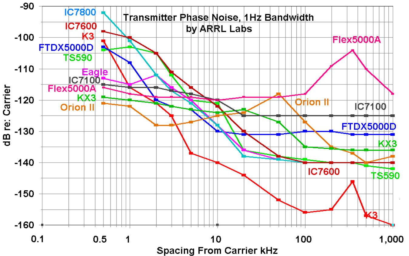
Figure 9 – Phase Noise 1 MHz Either Side of Carrier
