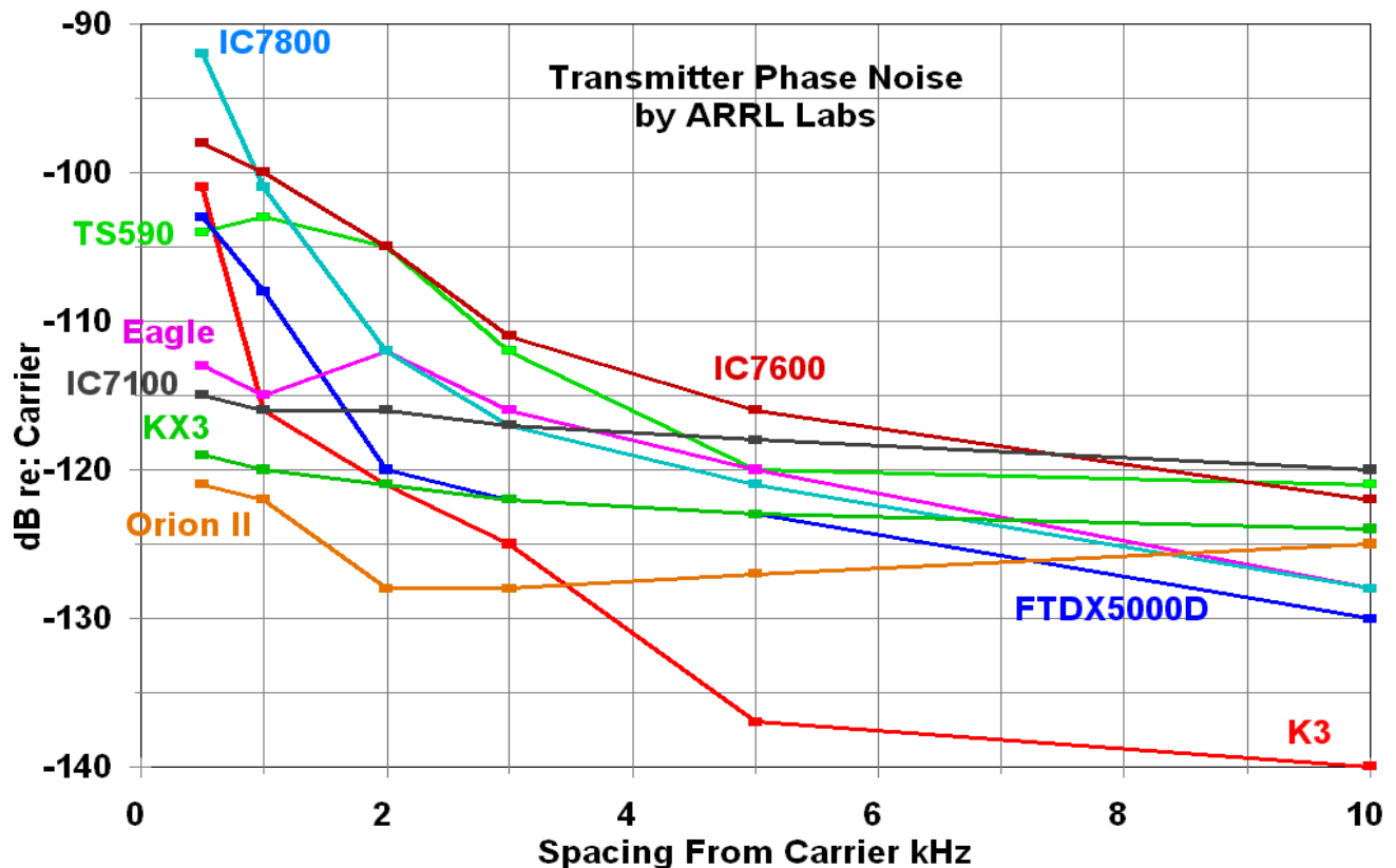
Figure 8 – Phase Noise Close To the Carrier
