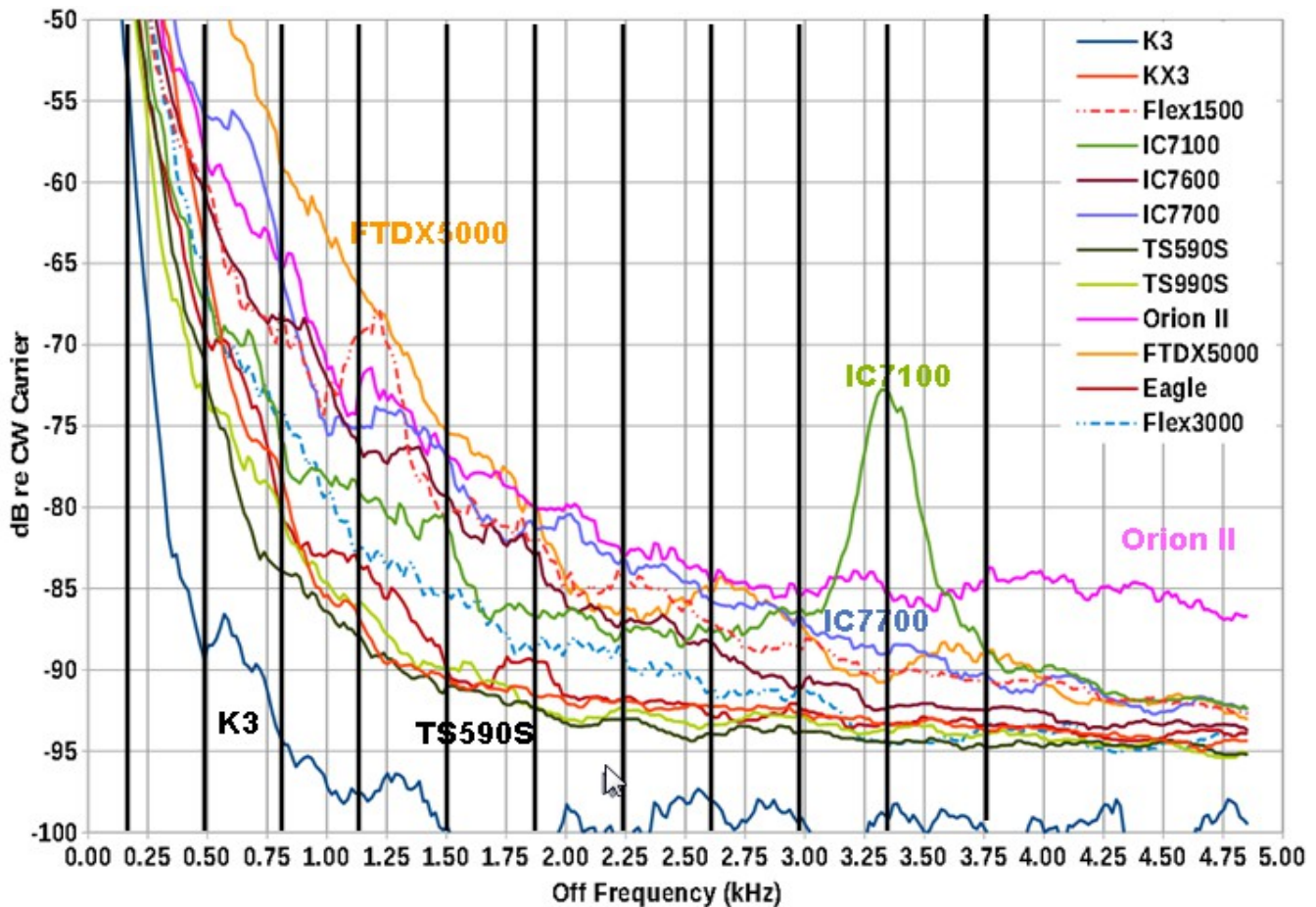
Figure 6 – 350 Hz Wide “Channels”
