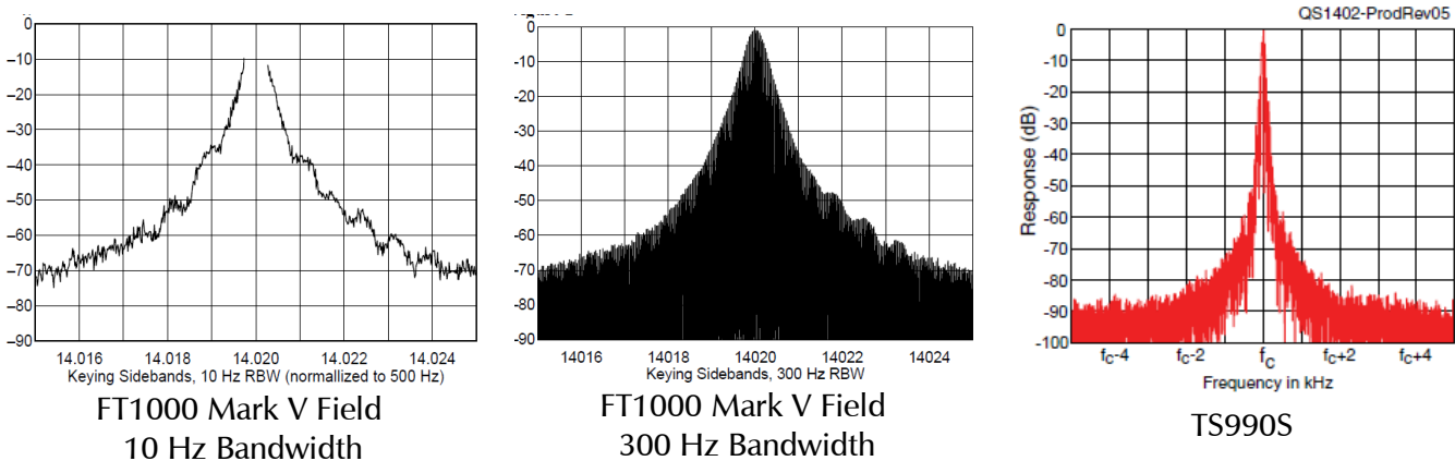
Figure 1 – The Raw Data
