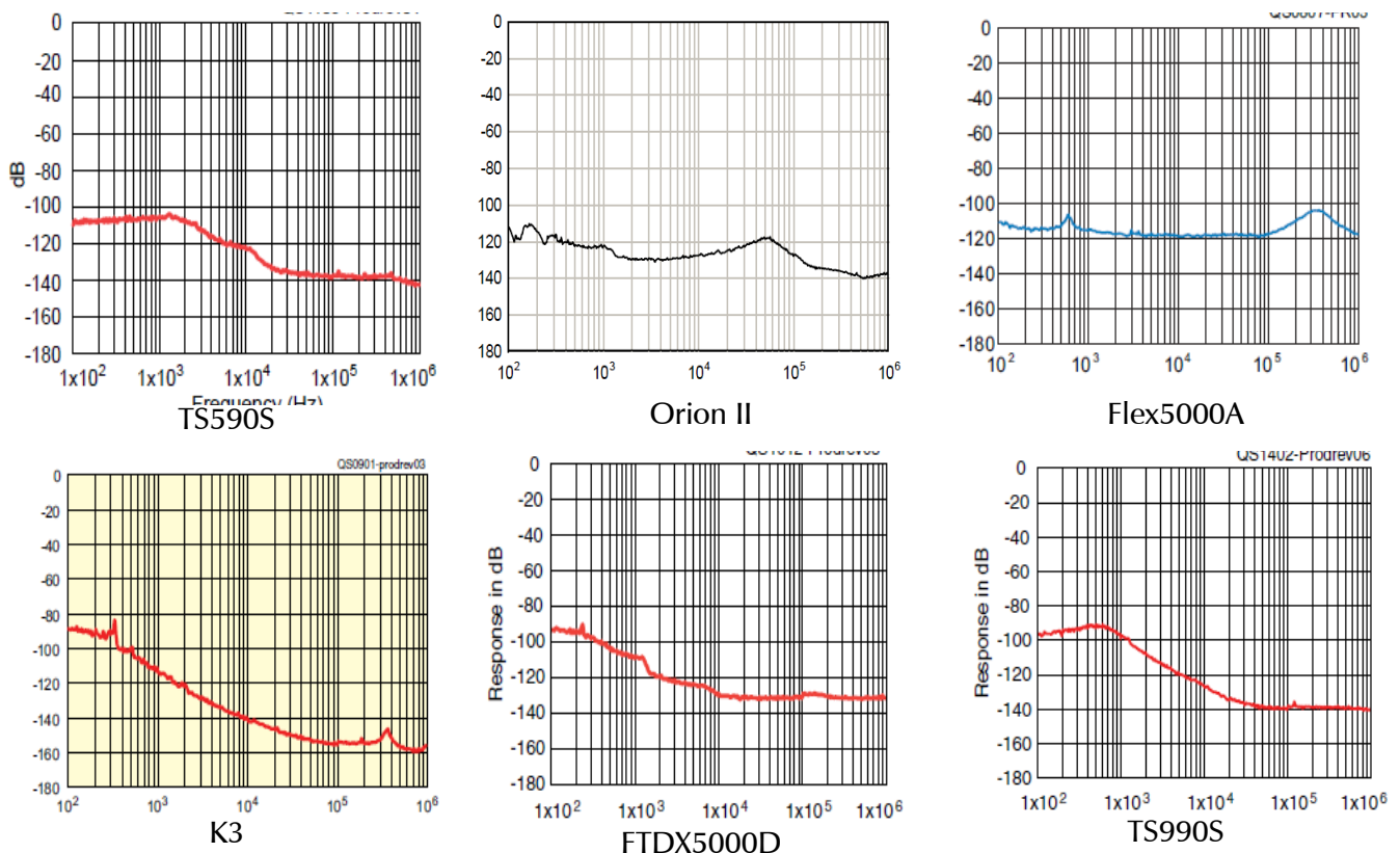
Figure 11 -- Selected Raw ARRL Lab Phase Noise Data
