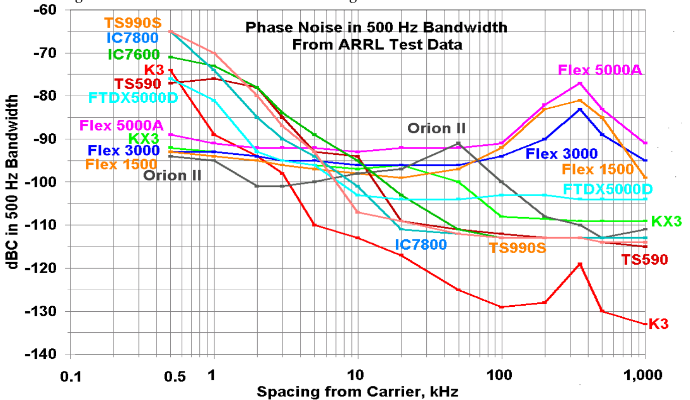
Figure 10 – Phase Noise Either Side of a Carrier
